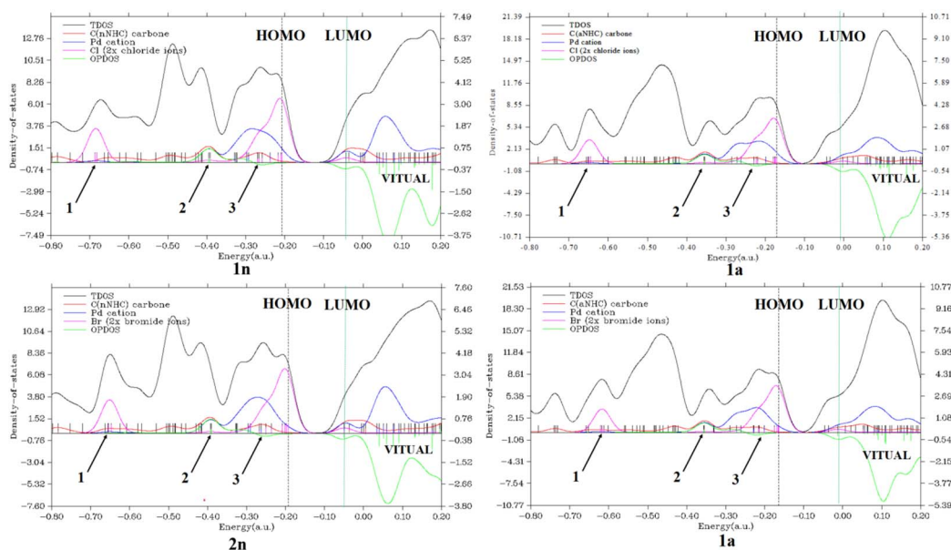
Fig. 4 . Total (black), partial [red ( C_{nNHC} ), blue ( Pd^{2+} ), and magenta ( Cl/Br )], and overlap [green, between C_{nNHC} and Pd^{2+} or Pd^{2+} and X(X = Cl/Br) basis functions] density-of-states map of bis(aNHC)[bis(nNHC)] Pd^{II}/Pd^{2+} complexes.
