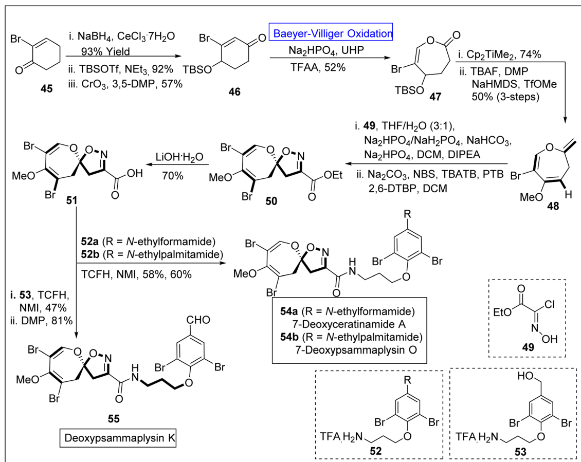
Scheme 7 Synthesis of deoxyxpsammapplysins O 54b , K 55 and deoxyceratinamide A 55 via Baeyer-Villiger oxidation.
