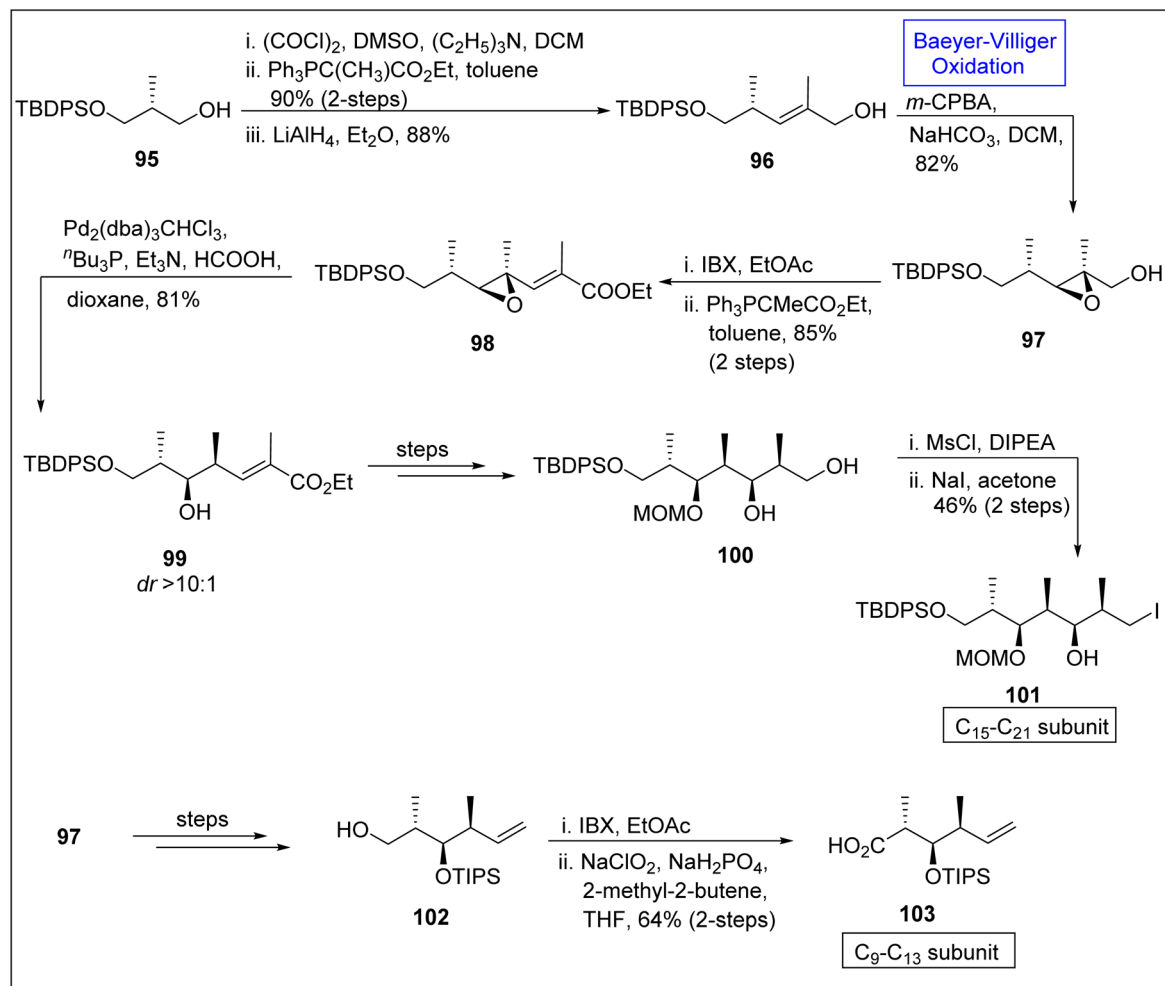
Scheme 12 Synthesis of C 15 -C 21 101 and C 9 -C 13 103 subunits of (+)-discodermolide via Baeyer-Villiger oxidation.
