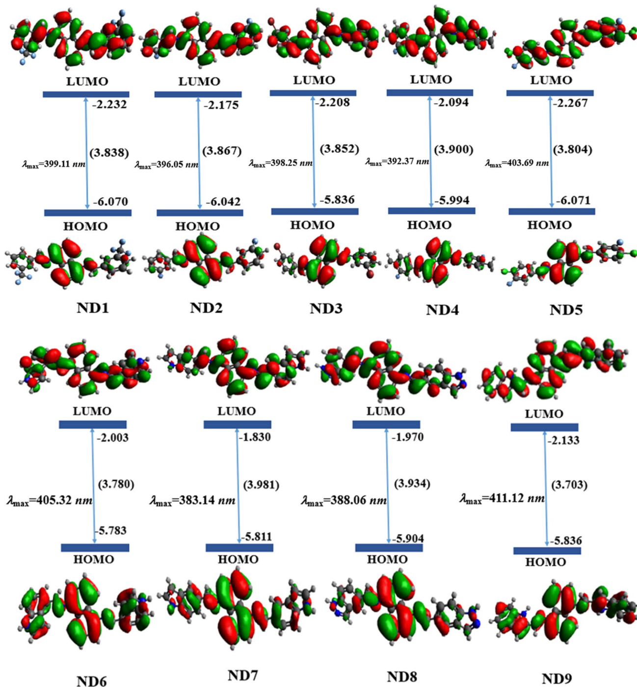
Fig. 1 Pictographic representation of charge distribution on HOMO and LUMO along with molecular orbital energies (in eV) of studied molecules.
