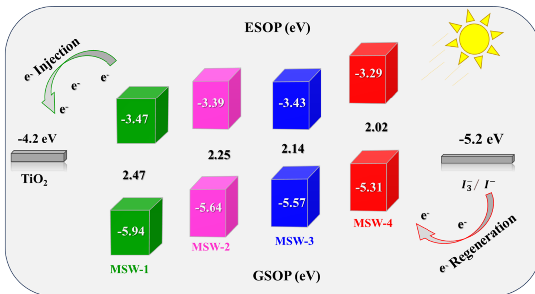
Fig. 6 Energy level diagram of the benzoxalacetonitrile sensitizer MSW-1-4 .
