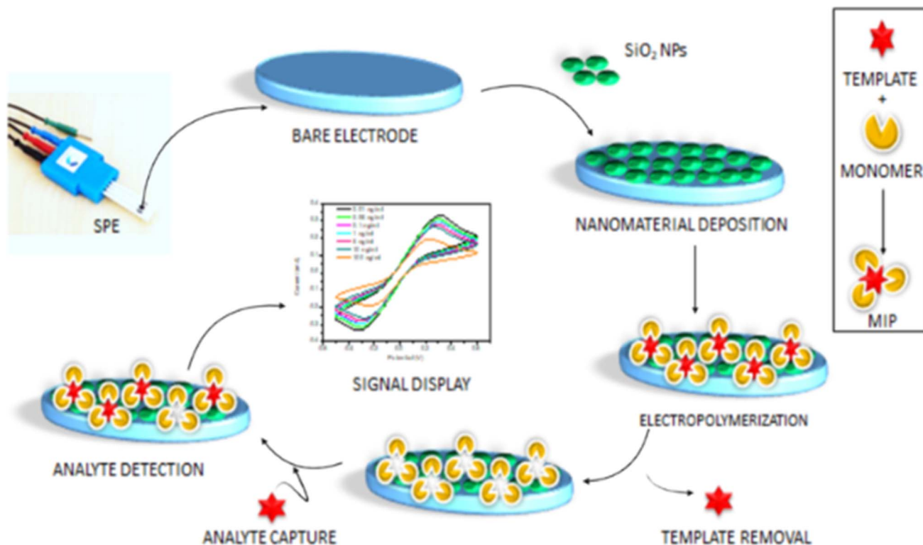
Fig. 13 Molecularly imprinted polymer (MIP) based biosensor. The figure was adapted from ref. 201 and reproduced with permission, copyright © Elsevier.
