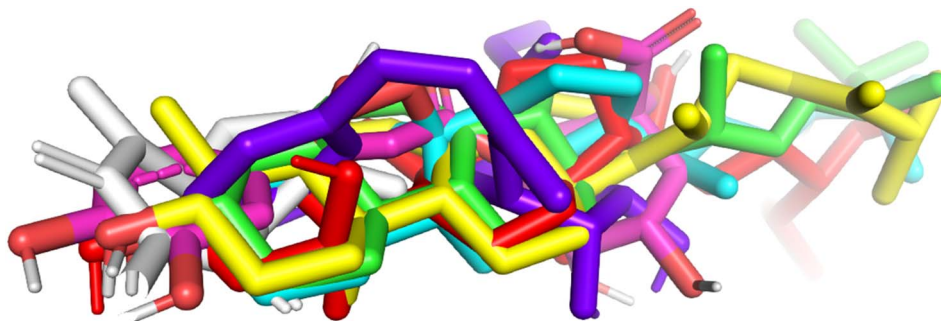
Fig. 6 The poses of compounds aligned to the pose-235, compound 7.
