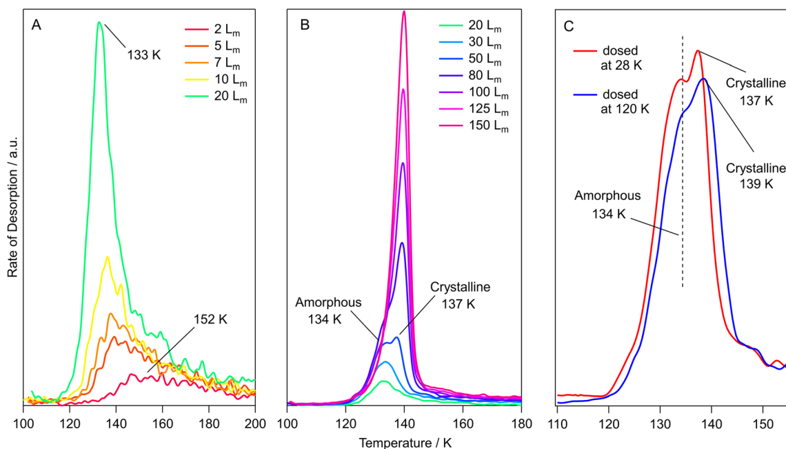
Fig. 5 TPD data for varying exposures of methyl propanoate adsorbed on HOPG. (A) Exposures from 2 L_m – 20 L_m dosed at 28 K. (B) Exposures from 20 L_m – 150 L_m dosed at 28 K. (C) A comparison of 50 L_m methyl propanoate ices grown at 28 K and 120 K.
