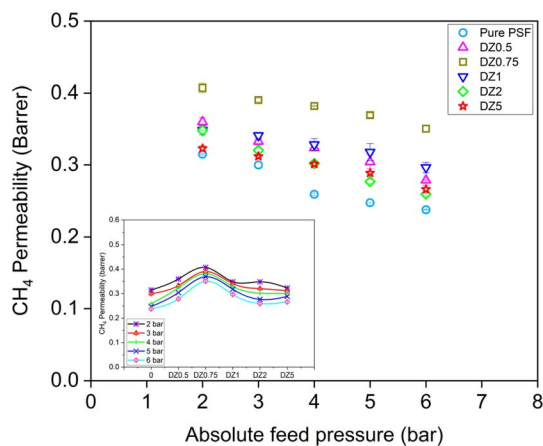
Fig. 9 CH 4 permeability of dense PSF/ZIF-8 mixed matrix membranes at different loadings of ZIF-8. Pure PSF results are also shown for comparison inset shows the permeabilities plotted as a function of loading for different pressures.
