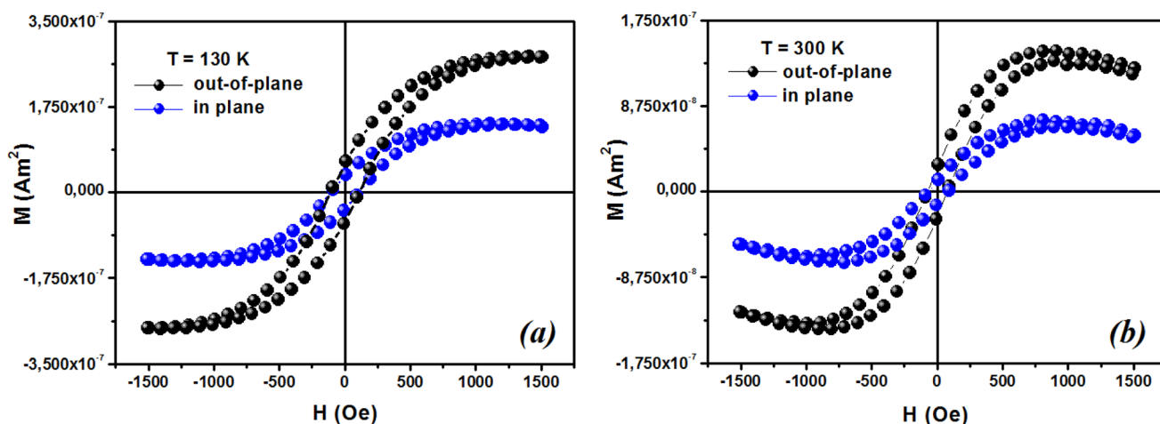
Fig. 13 Typical magnetic hysteresis loops of ZCO thin films in the range of 0° (out-of-plane) and 90° (in-plane) at (a) 130 K and (b) 300 K.
