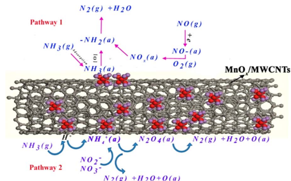
Fig. 15 Schematic diagram of two reaction pathways on MnO x /MWCNTs catalyst at 210 °C (reprinted from ref. 119. Copyright 2015, with permission from AAGR Aerosol and Air Quality Research).
