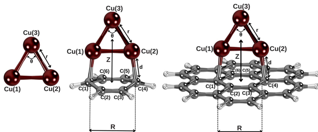
Fig. 1 Complexes under investigation at the equilibrium geometries (see Section 2 and the ESI† for the computational details). Z is defined as the distance between the centers of mass of Cu 3 and the benzene and coronene molecules, lying along the plotted axis.
