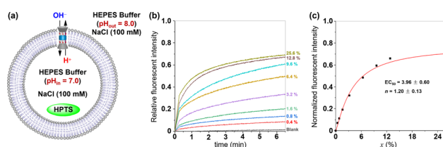
Fig. 5 (a) Schematic representation for the HPTS assay under alkaline condition. (b) Changes in the relative fluorescence intensity of HPTS (λ ex = 460 nm, λ em = 510 nm) in vesicles with time in the presence of varying concentrations of 1 (molar ratio relative to lipid, represented by x ). (c) Changes in normalized fluorescent intensity of HPTS in vesicles with the concentration of 1. Curve-fitting analyses were carried out by the Hill equation.
