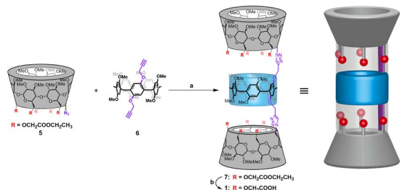
Fig. 2 Synthesis and structural features of channel 1: (a) CuSO 4 ·5H 2 O, sodium ascorbate, DMSO, r.t.; (b) LiOH·H 2 O, MeOH/H 2 O, r.t.
