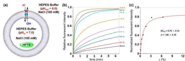
Fig. 4 (a) Schematic representation for the HPTS assay. (b) Changes in the relative fluorescence intensity of HPTS (λ ex = 460 nm, λ em = 510 nm) in vesicles with time in the presence of varying concentrations of 1 (molar ratio relative to lipid, represented by x ). (c) Changes in normalized fluorescent intensity of HPTS in vesicles with the concentration of 1. Curve-fitting analyses were carried out by the Hill equation.
