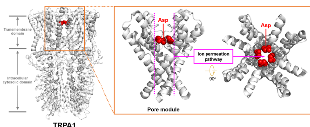
Fig. 1 Structural features of TRPA1.
