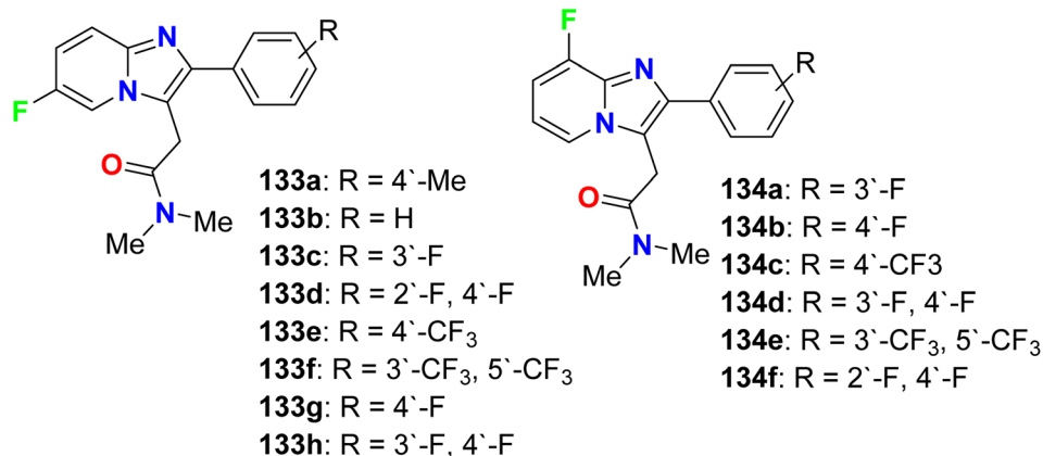
Fig. 74 Structure of 6-fluoro- and 8-fluoro-imidazo[1,2- a ]pyridine derivatives 133 and 134.
