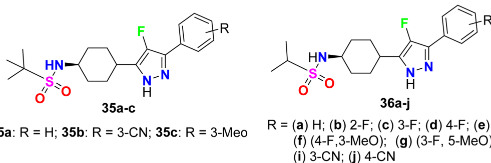
Fig. 24 Structure of 4-fluoropyrazole scaffolds 35a–c and 36a–j.
