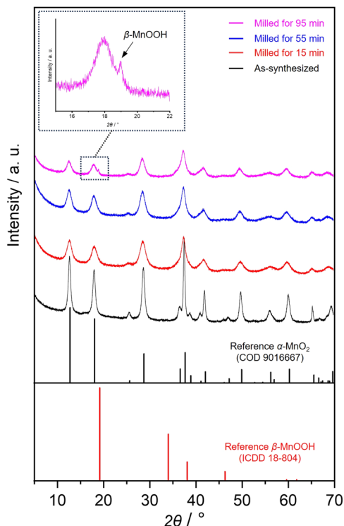
Fig. 1 PXRD patterns of as-synthesized and milled OMS-2 for different periods. Black arrow at 19.1^\circ indicates a 00 l reflection of feitknechtite, \beta -MnOOH.
