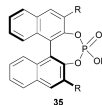
R : a = H, b = 4-nitrophenyl, c = 3,5-bis(trifluoromethyl)phenyl, d = 2,4,6-trimethylphenyl, e = naphthalen-2-yl, f = 2,4,6-tri(propan-2-yl)phenyl
