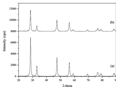
Fig. 2 XRD diffractograms of the flower-like \text{CeO}_2 catalyst: (a) before and (b) after reaction.
