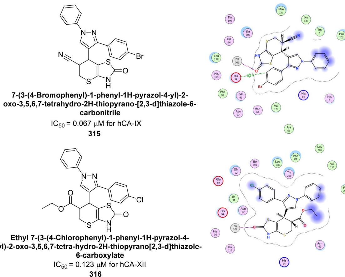
Fig. 114 Chemical structures of compounds 315 and 316; their K_i values against hCA-IX and XII along with their docking images.
