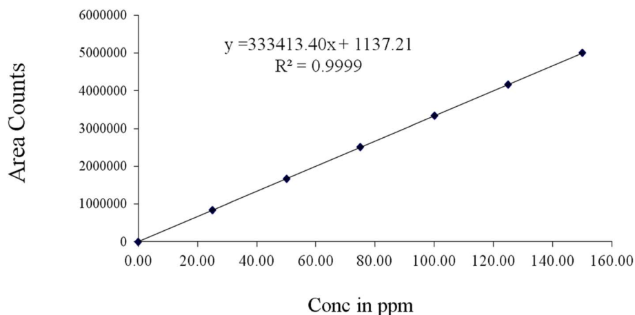
Fig. 4 Calibration curve for pirtobrutinib.
