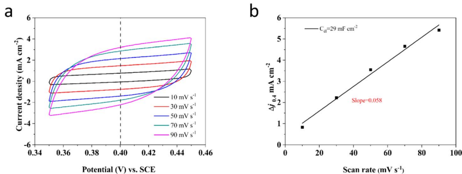
Fig. 8 (a) CVs of Ni-10.84 wt% Mo tested in a non-faradaic region of the voltammogram in 1 M KOH at different rates from 10 to 90 \text{mV s}^{-1} . (b) The corresponding capacitive current at 0.40 vs. SCE as a function of scan rate for as-deposited samples.
