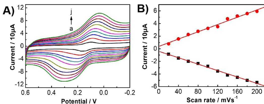
Fig. 6 (A) CVs of Bn on UCNPs-3DG/GCE in 0.1 M PBS under different scan rates in 0.1 M PBS (pH 7.0). (B) Redox peak current of Bn vs. scan rate. (a) 20 \text{ mV s}^{-1} , (b) 40 \text{ mV s}^{-1} , (c) 60 \text{ mV s}^{-1} , (d) 80 \text{ mV s}^{-1} , (e) 100 \text{ mV s}^{-1} , (f) 120 \text{ mV s}^{-1} , (g) 140 \text{ mV s}^{-1} , (h) 160 \text{ mV s}^{-1} , (i) 180 \text{ mV s}^{-1} , and (j) 200 \text{ mV s}^{-1} .
