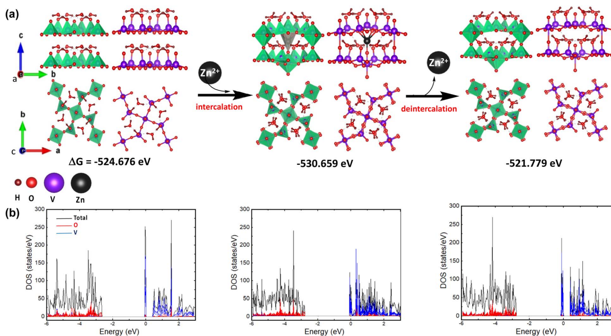
Fig. 7 (a) DFT-optimized geometries of layered V_3O_5(H_2O)_2 for the Zn^{2+} intercalation/deintercalation process, (I) pristine for the first charging/discharging step, (II) intercalated, (III) deintercalated; (b) total and partial DOS of I, II, and III.
