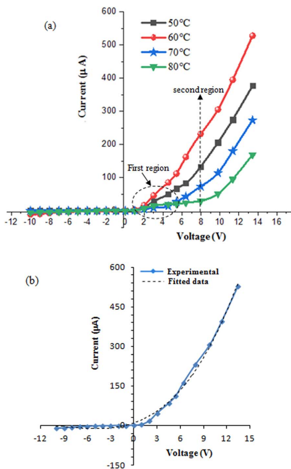
Fig. 14 (a) Dark I - V characteristics of n - \text{FeS}_2 / p - \text{Si} heterojunctions prepared at various deposition temperatures and (b) experimental and fitted I - V curves for heterojunction deposited at T_d = 60 °C.
