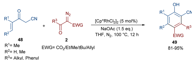
Scheme 23 Rh-catalyzed annulation of diazo compounds with 3-oxopent-4-enenitriles.
