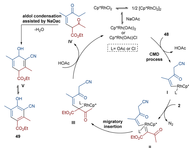
Scheme 24 Possible mechanism for the Rh-catalyzed annulation of diazo compounds with 3-oxopent-4-enenitriles.
