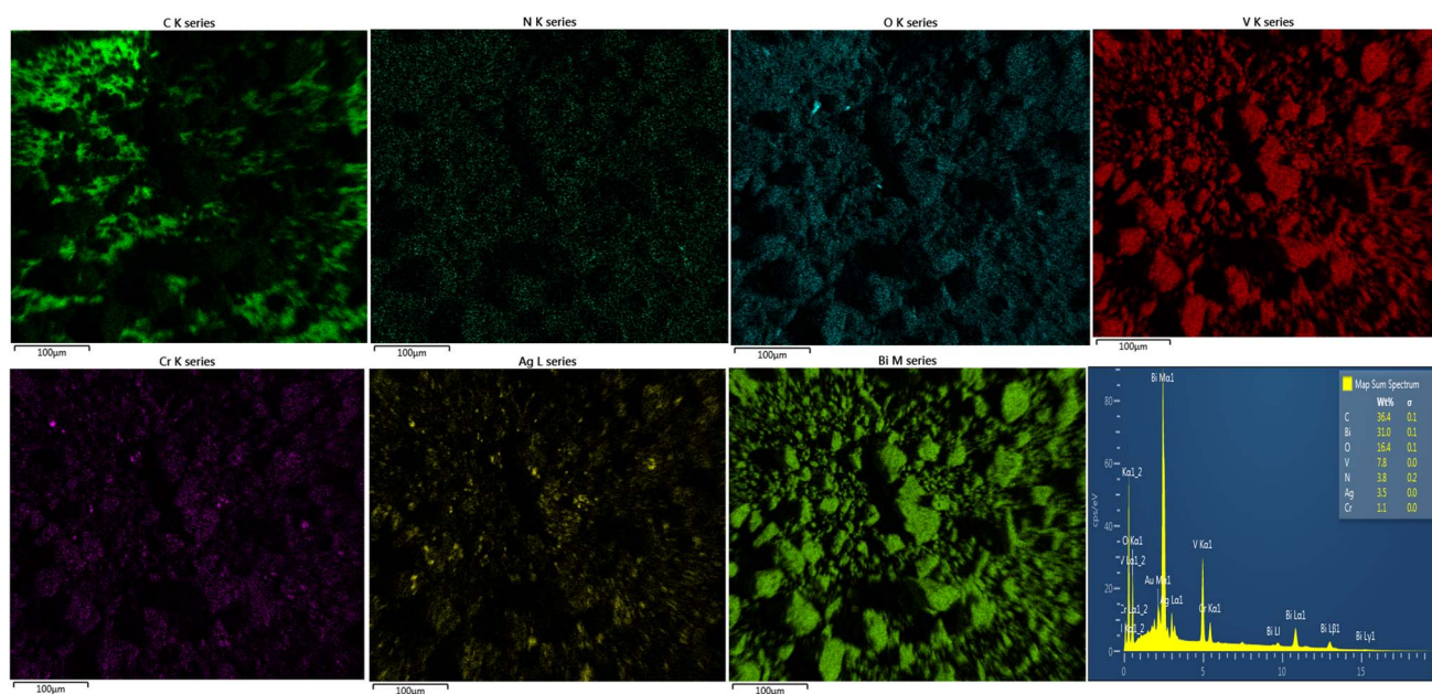
Fig. 3 Elemental mapping and EDS spectra of \text{GO}/\text{BiVO}_4/\text{Ag}_2\text{CrO}_4 nanocomposites.
