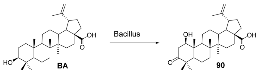
Fig. 27 Synthesis of BA derivative 90.
