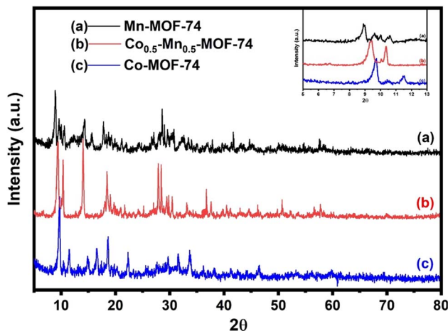
Fig. 1 XRD patterns of monometallic and bimetallic MOF-74.
