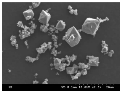
Fig. 11(a) SEM image for solid precipitate at 120 °C – H 2 O control group.
