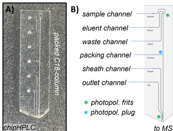
Fig. 6 Borosilicate glass chipHPLC with integrated injection cross, packed separation column, and monolithic electro spray emitter (as we presented before). A) Photograph of a fully manufactured chip. B) Schematic sketch of the chipHPLC describing all inlets and modifications for integration of the separation column (detailed information can be found in the ESI† section S1.2).
