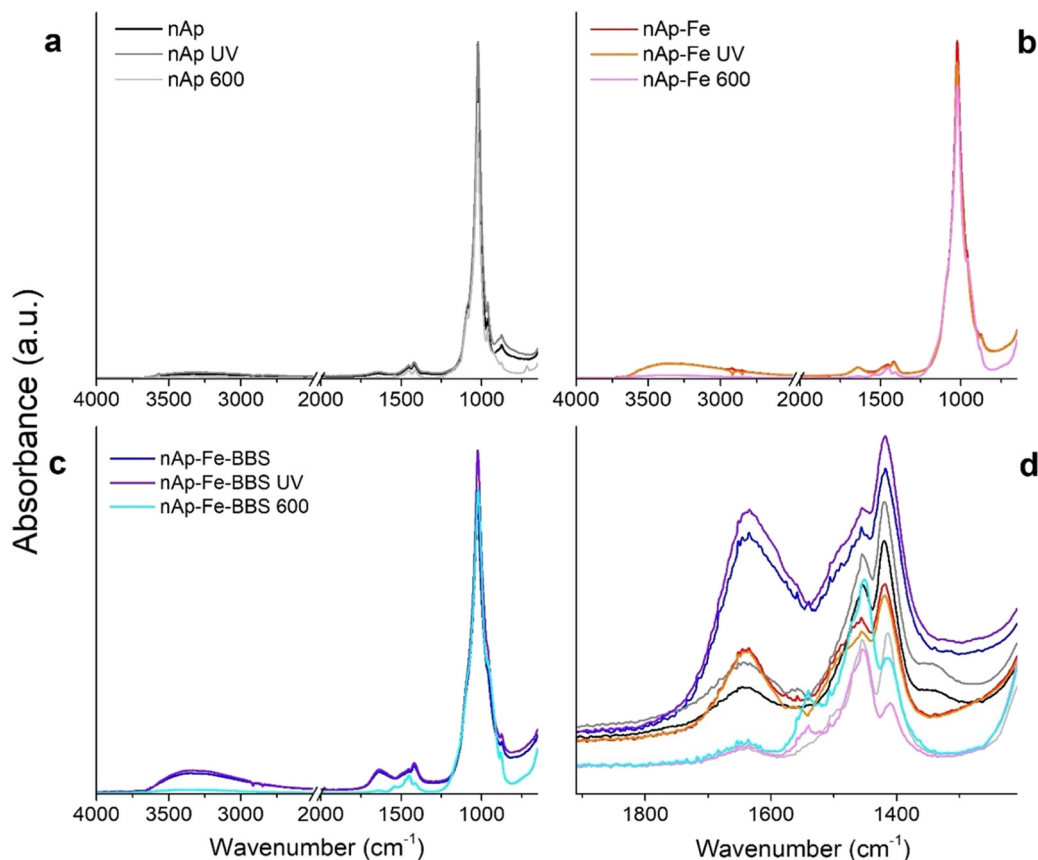
Fig. 3 ATR-FTIR spectra of different samples of as-prepared, UV-treated and calcined nAp (a), nAp-Fe (b) and nAp-Fe-BBS (c); in (d), the zoomed-in region of 1900–1200 cm -1 is reported for all the samples.
