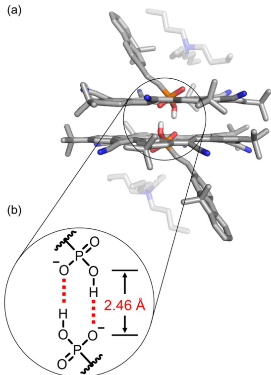
Fig. 3 (a) Crystal structure of 2 : 2 cyanostar : phosphonate complex with 9 with the presence of two tetrabutylammonium cations. (b) The pair of self-complementary hydrogen bonds are observed at a O...O distance of 2.46 Å. Data collected at 150 K. Non-polar hydrogen atoms and disorder of cyanostar and phosphonate omitted for clarity (CCDC 2263985).
