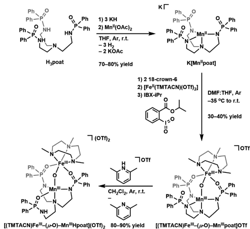
Scheme 2 Preparative routes for \text{K}[\text{Mn}^{\text{II}}\text{poat}] , \text{[(TMTACN)Fe}^{\text{III}}\text{-(}\mu\text{-O)-Mn}^{\text{III}}\text{poat]OTf} , and \text{[(TMTACN)Fe}^{\text{III}}\text{-(}\mu\text{-O)-Mn}^{\text{III}}\text{poat](OTf)}_2 .
