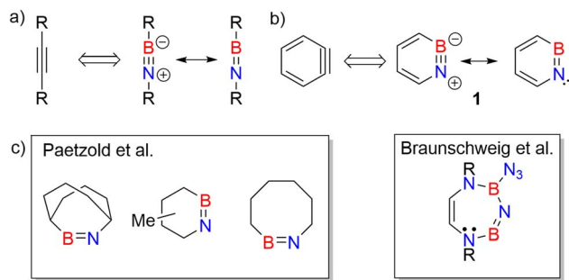
Scheme 1 (a) Iminoboranes and their analogy with alkynes. (b) Resonance forms of 1,2-azaborinine (1) and its analogy with ortho -benzyne. (c) Representative examples of cyclic iminoboranes previously inferred as reactive intermediates by Paetzold et al. 61 and Braunschweig et al. 42
