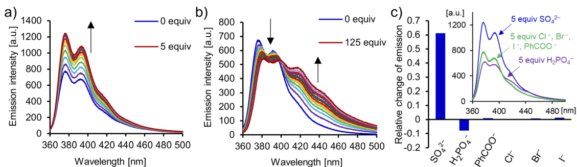
Fig. 9 Emission spectra recorded during titration of [2]catenane A with TBA 2 SO 4 (a) and TBAH 2 PO 4 (b) in DMSO/H 2 O 9 : 1 (ex: 350 nm). (c) Relative change of emission intensity: (I - I_0)/I_0 of catenane A at 370 nm in the presence of 5 equiv. of TBA salts of SO_4^{2-} , H_2PO_4^- , PhCOO^- , and halides ( Cl^- , Br^- , and I^- ) in DMSO/H 2 O 9 : 1 (ex: 350 nm). Inset: comparison of emission spectra of [2]catenane A in the presence of 5 equiv. of TBA salts of SO_4^{2-} , H_2PO_4^- , PhCOO^- , and halides ( Cl^- , Br^- , and I^- ) in DMSO/H 2 O 9 : 1 (ex: 350 nm).
