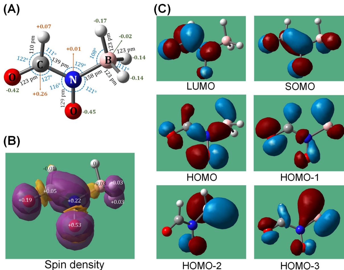
Fig. 5 (A) Optimized structure with Mulliken charges, (B) spin densities on the individual atoms and (C) selected molecular orbitals of the intermediate- N -boryl- N -oxo-formamide [HCON(O)BH 3 ] - ; BOFA radical anion formed in the initial reaction steps of [EMIM][CBH] and WFNA.
