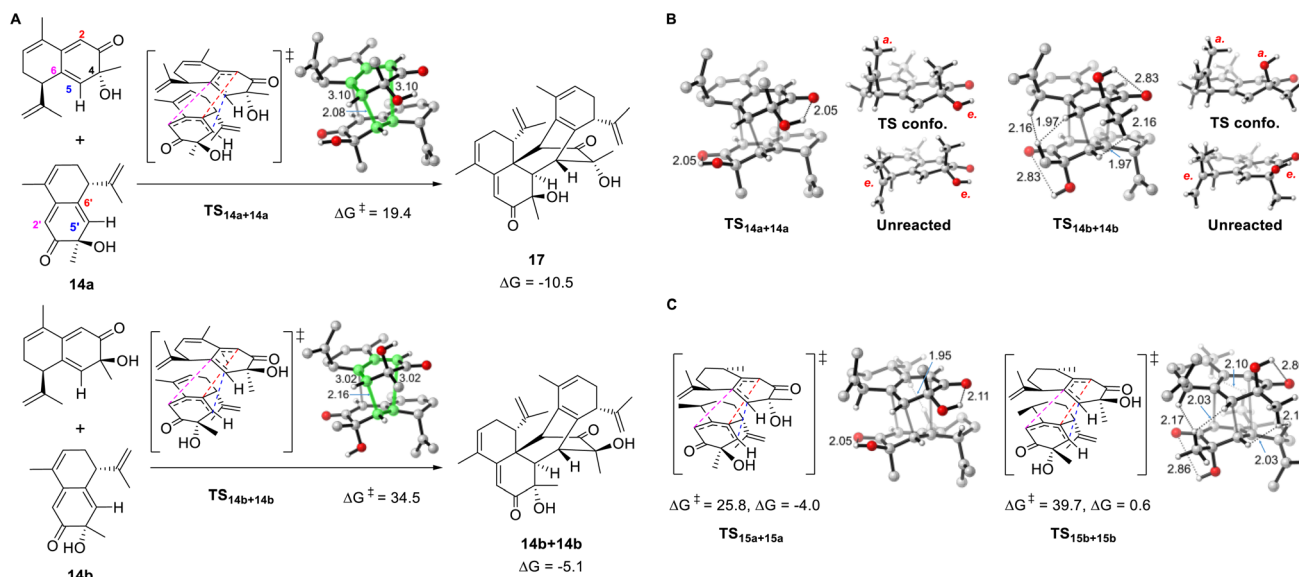
Fig. 4 Computational results. (A) Free energy barriers and reaction energies ( \text{kcal mol}^{-1} ) for the homo-dimerization reaction of 14a and 14b . (B) Comparison between TS_{14a+14a} and TS_{14b+14b} illustrates the origin of stereoselectivity. (C) Homo-dimerization reaction of 15a and 15b .
