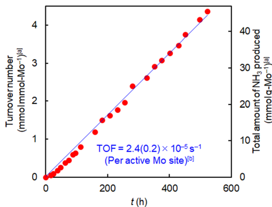
Fig. 3 Ammonia synthesis using (H 3 O) 2 [(Mo 6 Cl 8 )Cl 6 ]·6H 2 O ( 1 )/HY at 200 °C and 5.0 MPa (absolute pressure). Catalyst amount, 0.2 g; N 2 /H 2 (1/3-mixture) flow rate, 60 mL min -1 . [a] Per Mo included in the catalysts. [b] Per NH 3 -adsorbing Mo (see Table S4†).
