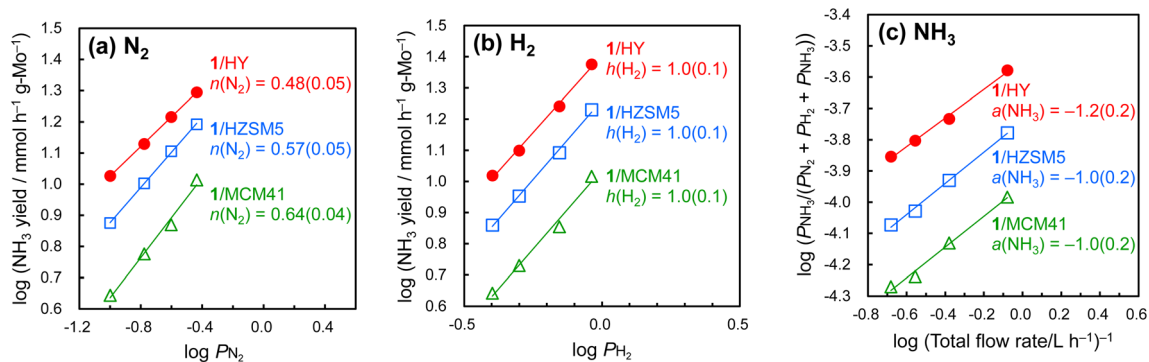
Fig. 4 Dependence of ammonia synthesis rate on the partial pressures of (a) N 2 , (b) H 2 , and (c) NH 3 over H 2 -activated clusters on various supports at 400 °C and 1 MPa.
