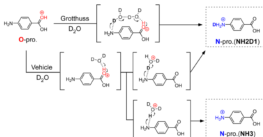
Fig. 1 Schematic illustration of hydration-induced \text{O} \rightarrow \text{N} proton transfer of \text{PABA}^+ by vehicle and Grotthuss mechanisms. The parentheses show a possible intermediate structure for the proton transfer. In the Grotthuss mechanism, proton transfer is mediated by a water bridge between CO and NH sites, resulting in a singly deuterated N-protomer denoted as NH2D1 . On the other hand, vehicle-type proton transfer affords both NH2D1 and nondeuterated NH3 . Note that the reaction intermediate in the scheme is simplified for clarity. For example, we do not exclude the possibility of bridged structures with more than two water molecules for the Grotthuss mechanism.
