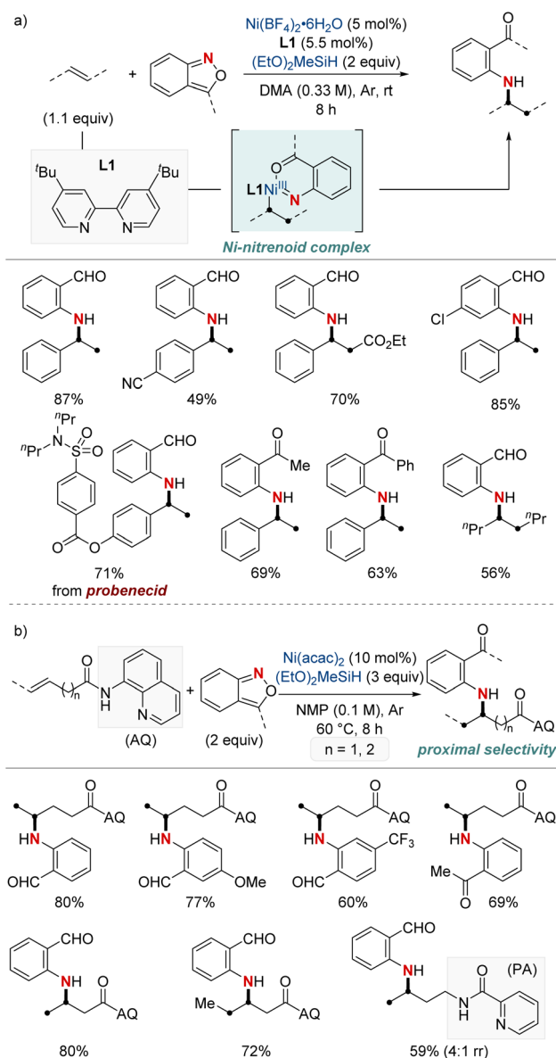
Scheme 3 (a) NiH-catalyzed hydroarylamination. (b) NiH-catalyzed hydroarylamination of unactivated alkenes.
