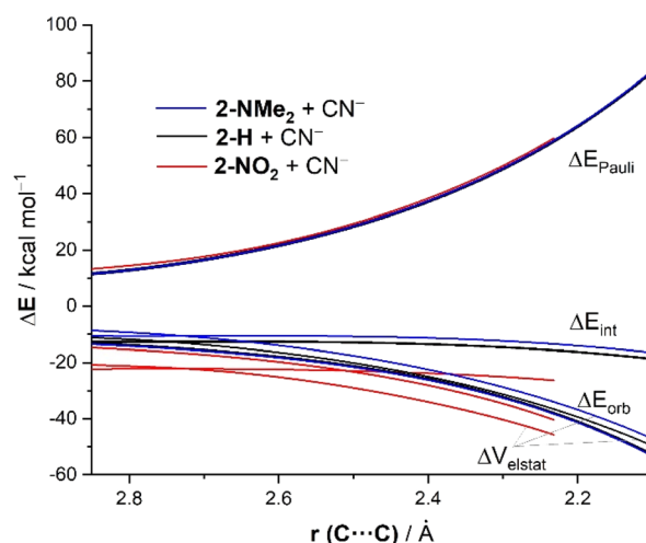
Fig. 7 Comparative EDAs of the reaction between \text{CN}^- and 2-NMe 2 (blue lines), 2-H (black lines) and 2-NO 2 (red lines) projected onto the C···C bond-forming distance and referred to the isolated reactants. All data have been computed at the ZORA-M06-2X/TZ2P//M06-2X/6-311+G* level.
