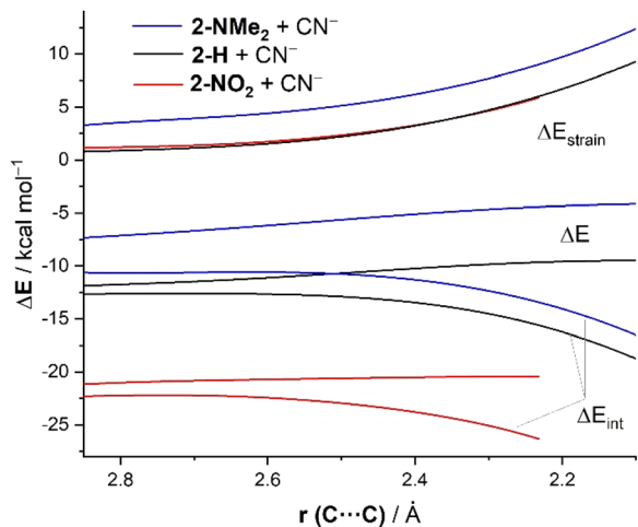
Fig. 5 Comparative ASDs of the reaction between \text{CN}^- and 2-NMe 2 (blue lines), 2-H (black lines) and 2-NO 2 (red lines) projected onto the C···C bond-forming distance and referred to the isolated reactants. All data have been computed at the ZORA-M06-2X/TZ2P//M06-2X/6-311+G* level.
