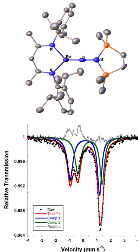
Fig. 5 (Top) ORTEP diagram of 8 with thermal ellipsoids shown at 50% probability and H atoms omitted for clarity; due to apparent disorder in the core, the structure is for connectivity only. (Bottom) Solid state zero-field Mössbauer spectrum of 8 at 80 K. The black circles are the data, the blue and green lines are the components of the fit, the red line is the sum of the components, and the grey line is the residual (data - fit).
