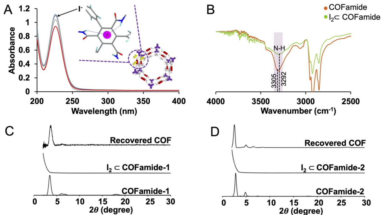
Fig. 3 (A) Adsorption of iodide in COFamide upon addition of \text{KI}_3 in water. Blue: \text{I}_2 saturated aqueous solution, t = 0 min, grey: t = every 5 min, red: t = 30 min (B) FT-IR of COFamide-2 (C) PXRD of COFamide-1 and (D) COFamide-2 before and after the iodine uptake.
