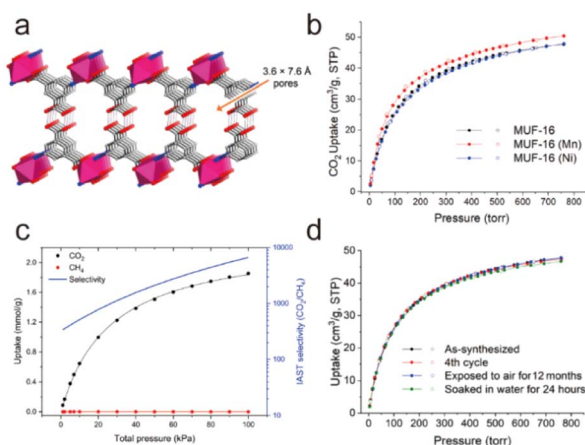
Fig. 44 (a) The structure of \text{MUF-16} . (b) The \text{CO}_2 adsorption isotherms of \text{MUF-16} s at 293 K. (c) The IAST selectivity of \text{MUF-16} for \text{CO}_2/\text{CH}_4 (50 : 50) at 293 K. (d) The \text{CO}_2 adsorption isotherms of \text{MUF-16} at 293 K, after 4 consecutive sorption cycles, 12 months of exposure to air with 80% RH, and 24 hours of immersion in water. Reproduced from ref. 265 with permission from Springer Nature, Copyright 2021.
