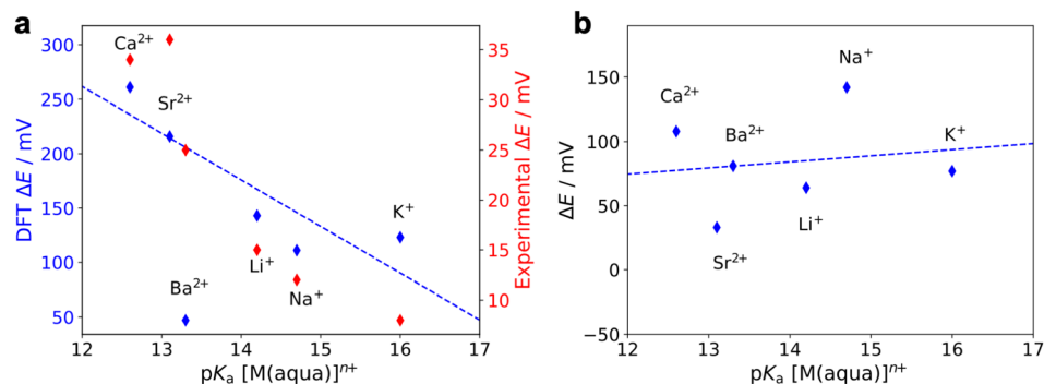
Fig. 11 Calculated relative reduction potentials (blue) of the \text{Co}^{\text{II}}/\text{Co}^{\text{I}} couple of \mathbf{1}^* when LAs are bound to the aza-crown ether as a function of the LA strength. These calculations were performed for (a) the most stable geometry ('folded', as shown in Fig. 10b) and (b) the geometry with an extended arm, as in Fig. S42.† \Delta E is the reduction potential for the \mathbf{1}^* -LA species relative to the reduction potential of \mathbf{1}^* with no LA bound in either the folded or extended arm geometry. An axial acetonitrile ligand was explicitly included for the \text{Co}^{\text{II}} species in these calculations. The data for \text{Ba}^{2+} is excluded in both linear fits. A second y axis in (a) shows the experimental values (red) measured via cyclic voltammetry.
