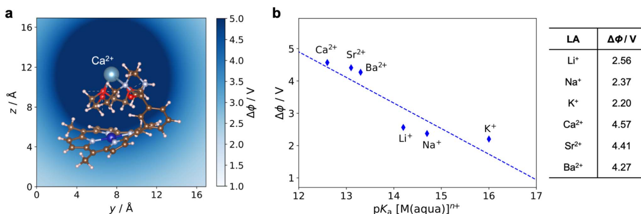
Fig. 12 (a) Electrostatic potential ( \Delta\phi ) generated by \text{Ca}^{2+} in \mathbf{1}^* - \text{Ca}^{2+} . (b) Calculated \Delta\phi generated by the LA at the Co center in \mathbf{1}^* -LA as a function of the LA strength.
