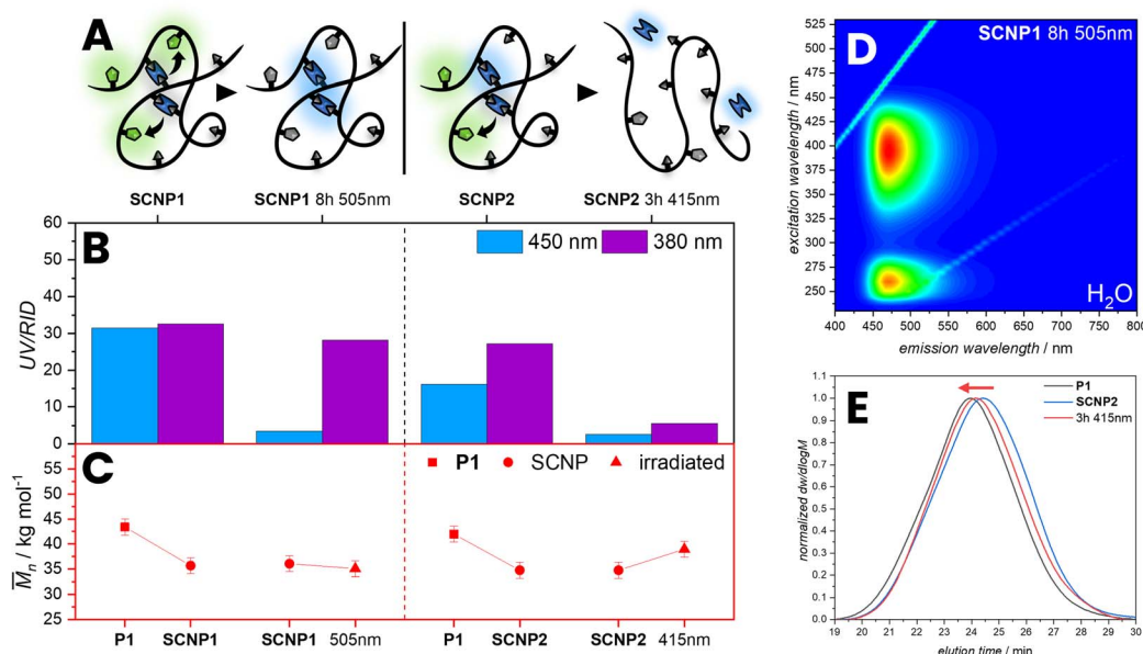
Fig. 5 (A) Illustration of SCNP1 irradiated with \lambda_{max} = 505 nm for 8 h resulting in photobleaching of the NBD and SCNP2 irradiated with \lambda_{max} = 415 nm for 3 h resulting in the cleavage and bleaching of the bimane units. (B) SCNP1 and SCNP2 analysed by SEC showing different absorption at 450 nm and 380 nm. (C) The apparent M_n (red) increases after irradiating with \lambda_{max} = 415 nm in water indicating unfolding of the SCNPs, whereas the apparent M_n does not increase after irradiating with \lambda_{max} = 505 nm. (D) 3D fluorescence spectrum of SCNP1 irradiated with 505 nm for 8 h in water. (E) RID SEC traces of SCNP2 unfolding compared to P1. M_n : apparent number average molecular weight.
