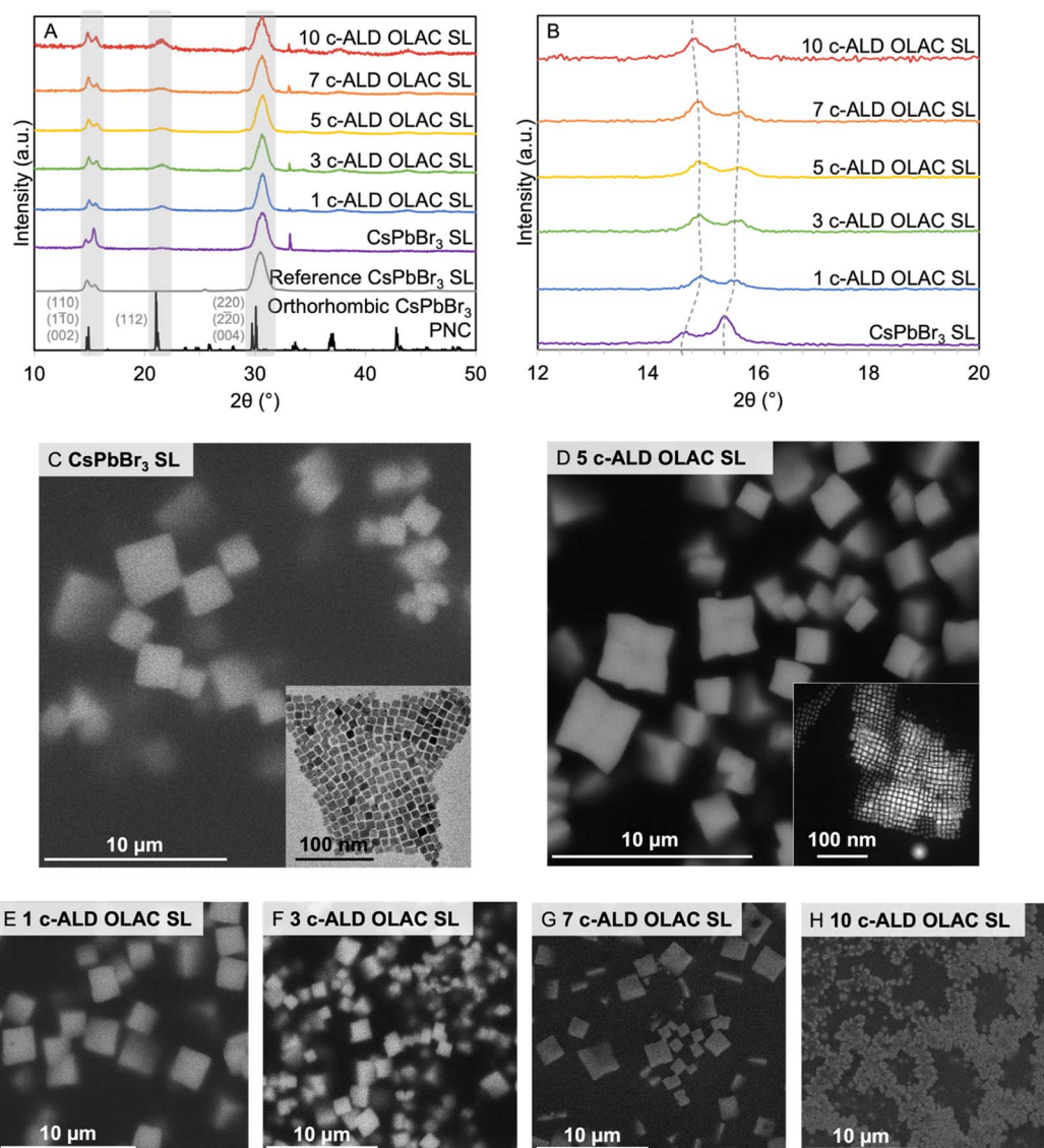
Fig. 2 (A) PXRD diffractograms of SLs constructed from untreated and c-ALD OLAC treated CsPbBr 3 PNCs (reference pattern for orthorhombic CsPbBr 3 PNCs from ICSD 97851, reference SL pattern from ref. 23), and (B) isolation of splitting at 15° 2 \theta . (C) SEM and (inset) TEM micrographs of CsPbBr 3 SLs and PNCs, respectively, (D) SEM and (inset) HAADF-STEM micrographs of 5 c-ALD OLAC SL and PNCs, respectively, (E) SEM-EDS mapping of 5 c-ALD OLAC SLs, and (F–I) SEM micrographs of corresponding c-ALD OLAC treated CsPbBr 3 SLs.
