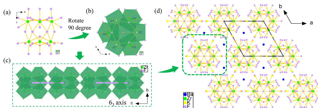
Fig. 1 (a and b) cis-[Zr_6F_{34}]^{10-} cluster at the ac and ab plane; (c) the \{[Zr_6F_{34}]^{7-}\}_\infty chain along the c -axis; (d) the aligned arrangement of the \{[Zr_6F_{34}]^{7-}\}_\infty anionic chains and whole structure of K_3Ba_2Zr_6F_{31} viewed along the c -axis.
