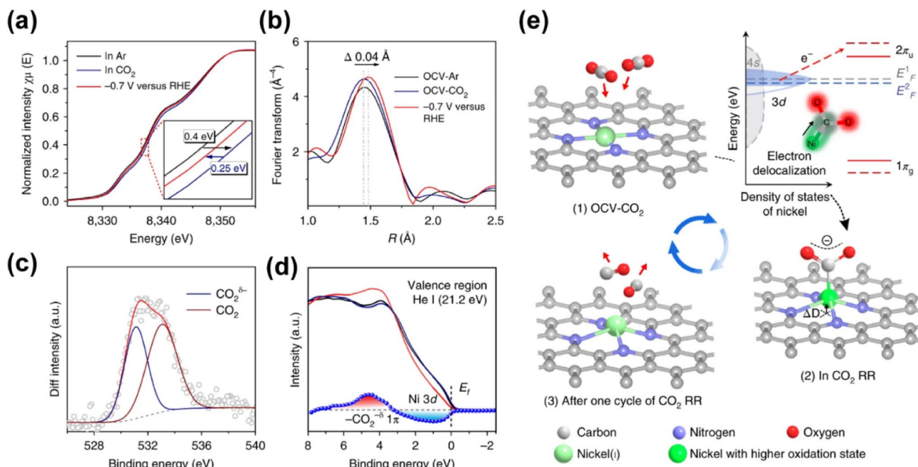
Fig. 15 (a) Normalized operando Ni K-edge XANES spectra for A-Ni-NG at various biases ( versus RHE) in 0.5 M KHCO 3 aqueous solution at room temperature and 1 atm of Ar or CO 2 . The inset shows the enlarged Ni K-edge XANES spectra. (b) Fourier transform magnitudes of EXAFS spectra (without phase correction) of A-Ni-NG under open-circuit voltage bias in Ar (OCV-Ar) and CO 2 (OCV-CO 2 ), and at -0.7 V ( versus RHE), in which an expanded Ni-N bond was detected. (c) Change in the XPS O 1s intensity induced by CO 2 adsorption for A-Ni-NG. (d) Valence band spectra of A-Ni-NG before (black line) and after (red line) CO 2 gas exposure, and after desorption of CO 2 by thermal treatment at 773 K for 20 min in a vacuum (dark blue line). The blue line shows the variation in the valence band spectra of A-Ni-NG induced by CO 2 adsorption. (e) Structural evolution of the active site in electrochemical CO 2 reduction. 140 Reproduced from ref. 140 with permission from Springer Nature, copyright 2018.
