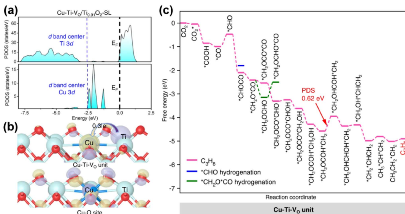
Fig. 32 (a) PDOS and d-band centres of Cu 3d and Ti 3d orbitals. (b) Charge density differences of the Cu–O site and Cu–Ti– V_O unit. (c) Gibbs free energy diagrams of CO_2 reduction on the Cu–Ti– V_O unit. 295 Reproduced from ref. 295 with permission from Springer Nature, copyright 2023.
