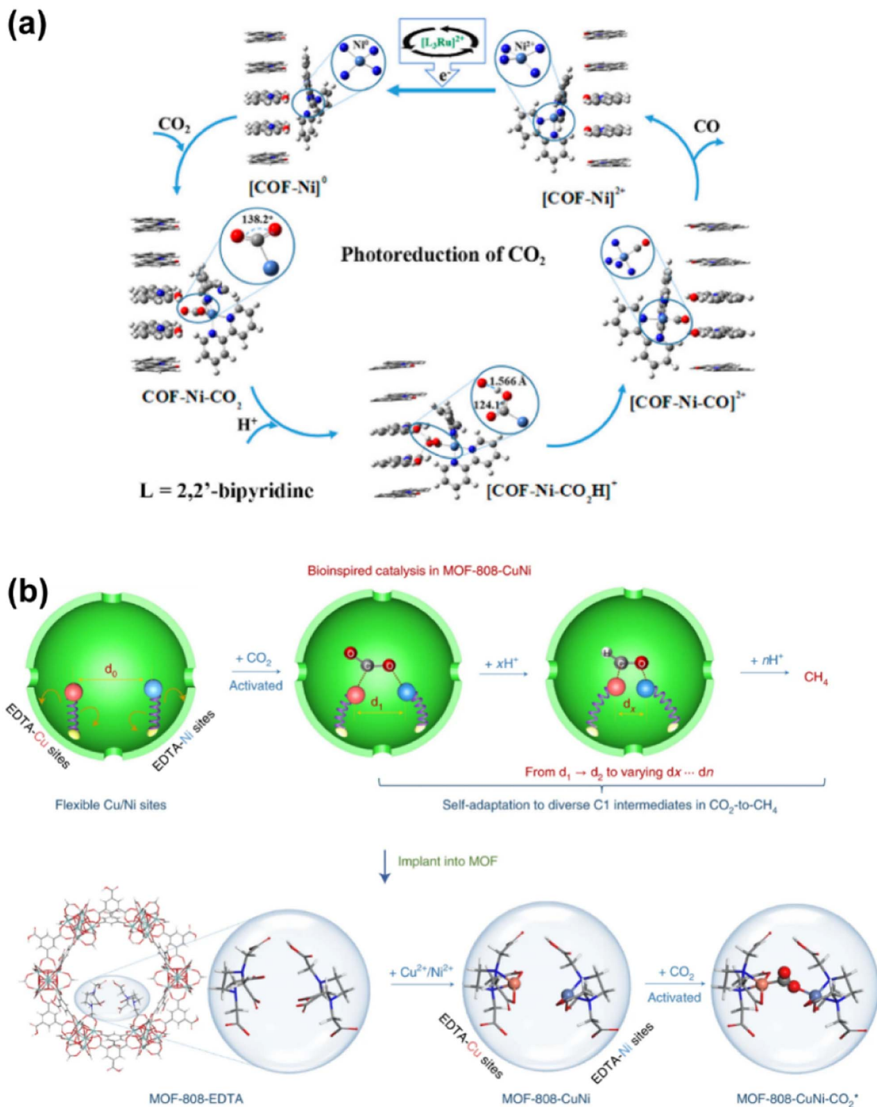
Fig. 27 (a) Proposed reaction mechanism for the photoconversion of CO 2 into CO on Ni-TpBpy. 267 (b) Implanting flexible and self-adaptive Cu/Ni DMSPs into MOF-808 for highly selective CO 2 photoconversion to CH 4 . 268 Reproduced from ref. 267 and 268 with permission from American Chemical Society and Springer Nature, copyright 2019, 2021.
