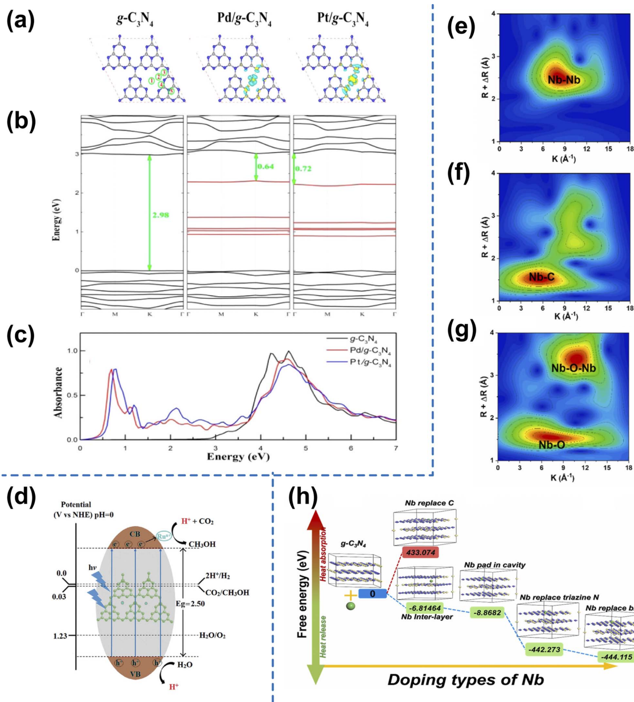
Fig. 26 (a) Optimized structure and plots of 3D differential charge densities, (b) band structures, and (c) optical absorption spectra of g\text{-C}_3\text{N}_4 , \text{Pd}/g\text{-C}_3\text{N}_4 , and \text{Pt}/g\text{-C}_3\text{N}_4 . 252 (d) Possible schematic representation of the photocatalytic mechanism over the \text{RuSA-mC}_3\text{N}_4 surface under visible light irradiation. 250 The WT-EXAFS plots of Nb-foil (e), \text{CNNb}_{0.06} (f), and \text{Nb}_2\text{O}_5 (g), respectively; free energy (h) of various possible modes of single-atom Nb using DFT calculations. 243 Reproduced from ref. 240, 243, 250 and 252 with permission from American Chemical Society, Wiley and Elsevier, copyright 2016, 2020, 2023.
