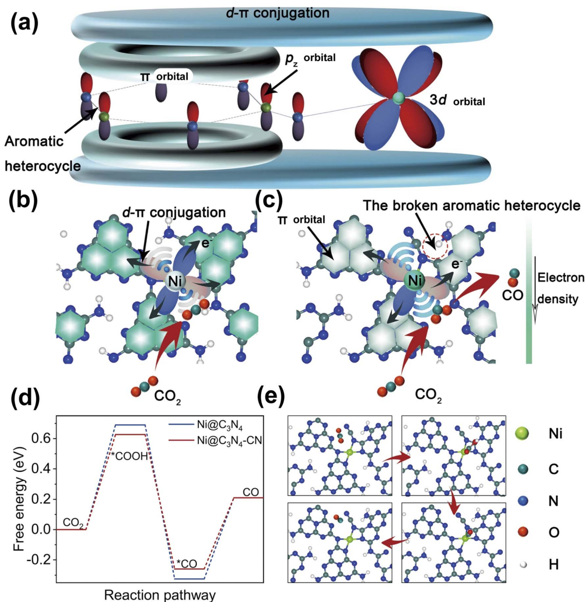
Fig. 47 (a) Schematic of d - \pi conjugation. The effect of d - \pi conjugation on CO 2 activation over (b) Ni-C 3 N 4 and (c) Ni-C 3 N 4 -CN. (d) Free energy diagram of CO 2 conversion to CO. (e) Structure and adsorption configurations of key intermediates on Ni-C 3 N 4 -CN. Reproduced from ref. 394 with the permission of Nature Springer, copyright 2022.
