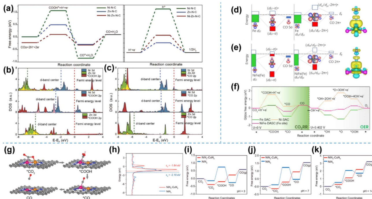
Fig. 20 (a) The free energy of each intermediate state on the metal atom sites in Zn-N 4 -C, Ni-N 4 -C, and ZnNi-N 6 -C. Projected DOS (PDOS) for Zn/Ni 3d orbitals and oxide 2p orbitals including COOH (b) and CO (c). 201 Schematic illustration of orbital interactions between adsorbed CO ( 5\sigma and 2\pi^* ) and the 3d orbital ( d_{z^2} , d_{xz}/d_{yz} ) of the Fe site in the (d) Fe-SAC and (e) NiFe-DASC. (f) Calculated free energy diagrams for \text{CO}_2 RR and OER processes. 203 (g) The catalytic pathway on NiN 3 -CuN 3 based on the ^*\text{COOH} and ^*\text{CO} adsorption intermediates after optimization. (h) The density of states of Ni d-orbitals in NiN 3 -CuN 3 and NiN 3 . (i–k) Gibbs free energy diagrams of \text{CO}_2 conversion to CO over NiN 3 -CuN 3 and NiN 3 with free energy correction at pH = 3, 7, and 14. 202 Reproduced from ref. 201–203 with permission from Wiley and Springer Nature, copyright 2021, 2023.
