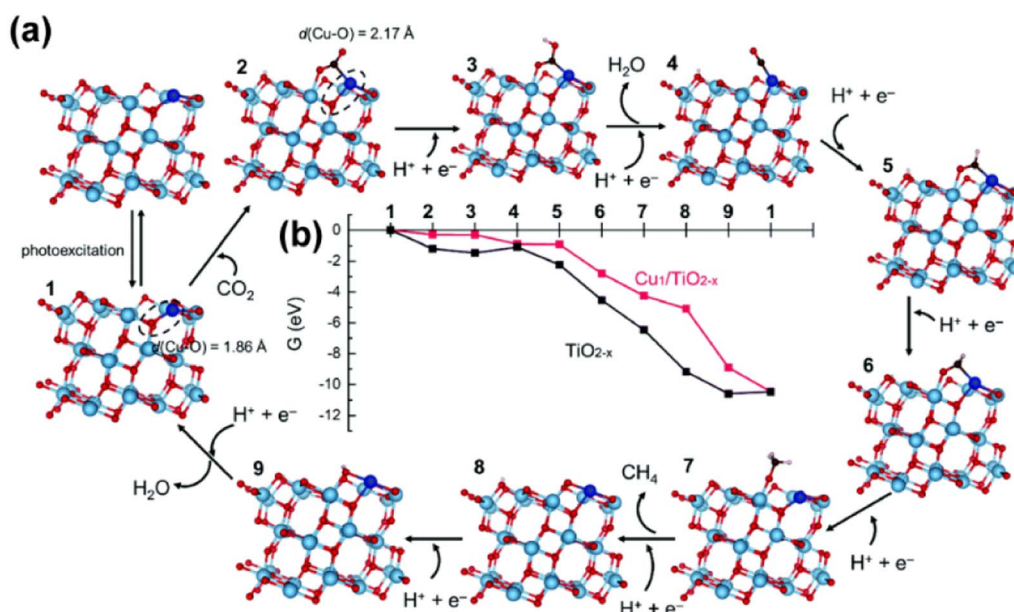
Fig. 24 Photocatalytic CO 2 reduction at Cu 1 /TiO 2-x with an oxygen vacancy. (a) CO 2 reduction mechanism at Cu 1 /TiO 2-x and (b) DFT energetics of CO 2 reduction at Cu 1 /TiO 2-x and TiO 2-x . During the reduction process, the photoexcited electron is assumed to be transferred from the conduction band minimum of TiO 2 (−0.25 V versus RHE). 231 Reproduced from ref. 231 with permission from Royal Society of Chemistry, copyright 2022.
