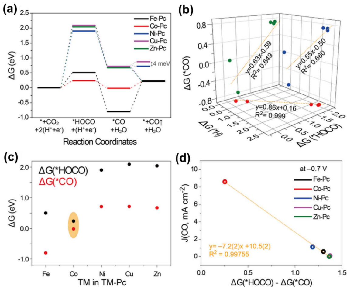
Fig. 37 Correlation between experimental results and theoretical calculations. (a) Free energy diagram for \text{CO}_2 reduction at E = 0 V. (b) Linear fitting between the free energy of reaction intermediates over different transition metals. (c) Free energy of ^*\text{HOCO} and ^*\text{CO} with different transition metals. (d) Plot of the free energy difference of ^*\text{HOCO} and ^*\text{CO} adsorption versus current density of \text{CO} production at -0.7 V. Reproduced from ref. 330 with the permission of American Chemical Society, copyright 2022.
