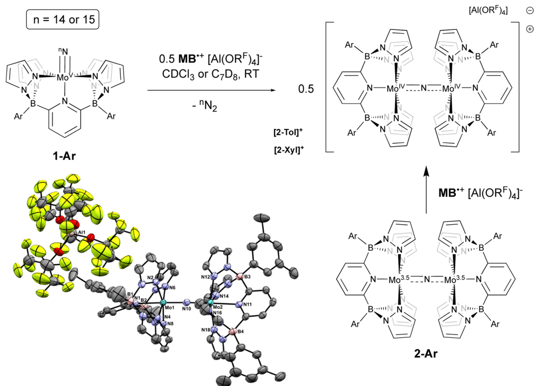
Fig. 3 Oxidation of neutral nitridos 1-Ar with 0.5 equivalents of [\mathbf{MB}]^+[\text{Al}(\text{OR}^F)_4]^- . Lower left: molecular structure of [\mathbf{2-Xyl}]^+[\text{Al}(\text{OR}^F)_4]^- . Thermal ellipsoids are shown at the 50% probability level and all H atoms are omitted for clarity. Selected bond distances (Å): Mo(1)–N(10), 1.856(3); Mo(2)–N(10), 1.859(3); Mo(1)–N(1), 2.260(3); Mo(2)–N(11), 2.265(3). Selected bond angles (°): Mo(1)–N(10)–Mo(2), 176.52(19).
