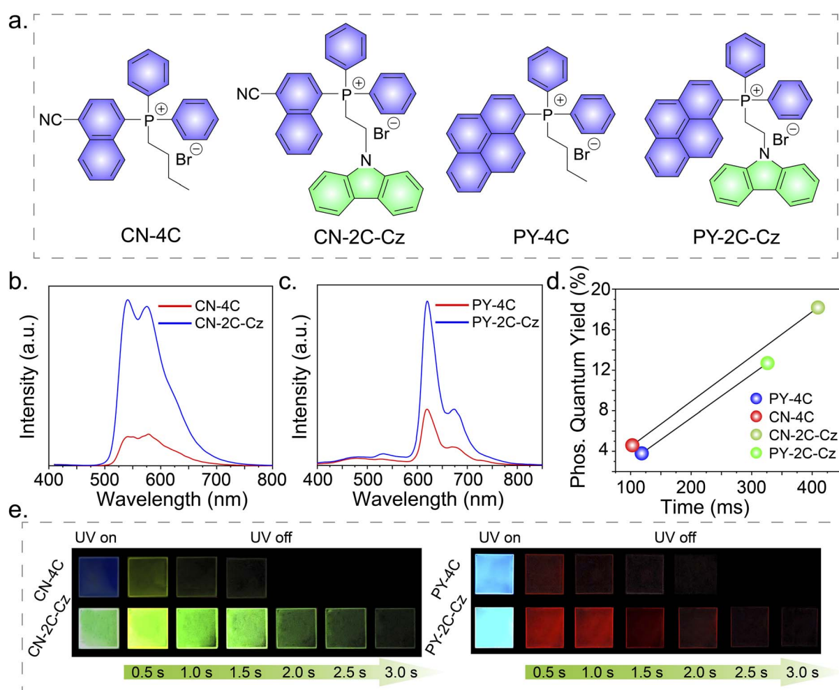
Fig. 4 (a) Molecular structures of CN-4C , CN-2C-Cz , PY-4C , and PY-2C-Cz . (b) The delayed PL spectra for PVA films doped with CN-4C and CN-2C-Cz (Ex = 300 nm). (c) The delayed PL spectra for PVA films doped with PY-4C and PY-2C-Cz (Ex = 300 nm). (d) Comparative evaluation of phosphorescence quantum efficiencies and lifetimes for each compound in PVA films. (e) Afterglow photos of compound-doped PVA films.
