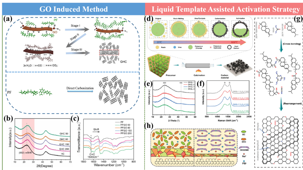
Fig. 7 (a) Proposed formation mechanism of GHCs under different conditions, (b and c) XRD patterns and FTIR spectra of GHCs, (d) diagram for the preparation of “egg puff”-like HC, (e and f) XRD patterns and Raman spectra of SNQLs, (g) diagram of the structure transformation and (h) diagram of SEI in different electrolytes.
